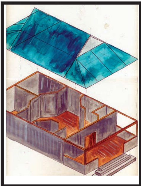
Exploded view of main floor
